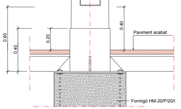
COLUMNA I PLAQUES BASE
