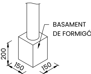
DETALL E 1/20 (A3) BASSAMENT PILONA
