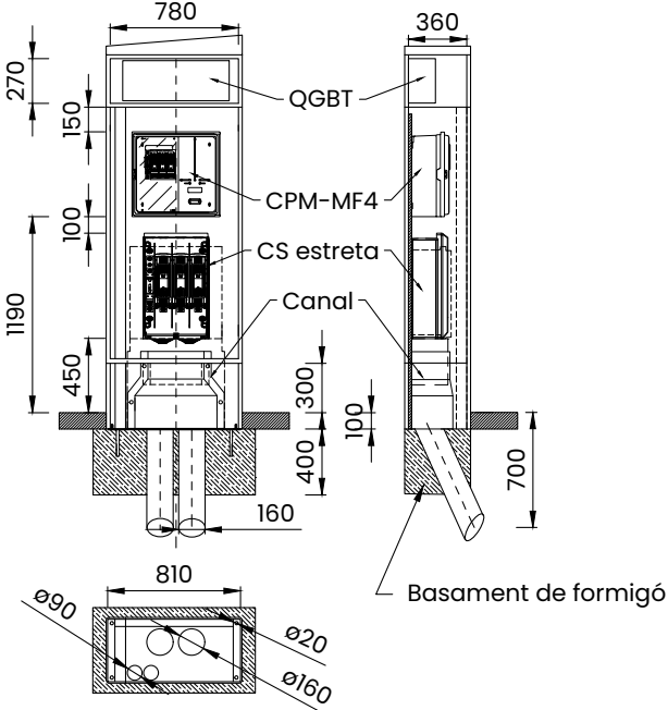
DETALL 1/50 (A3) MONOLIT CPM-MF4 <43,5 kW
